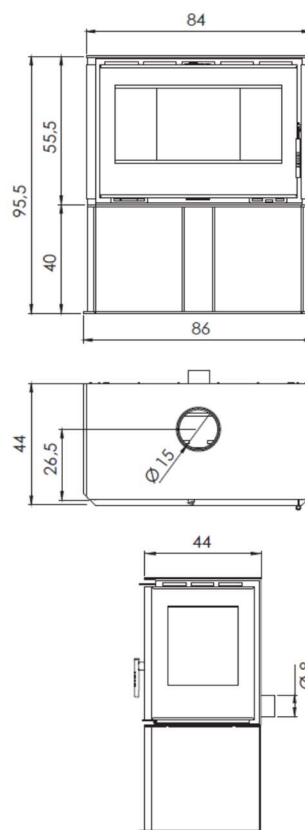
RA-85-2 LEÑERA RA-85-2 WITH LOG STORE
