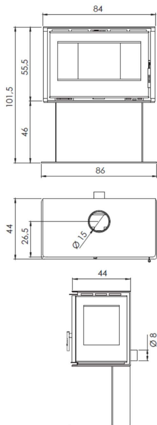
RA-85-2 PIE RA-85-2 FREE-STANDING
